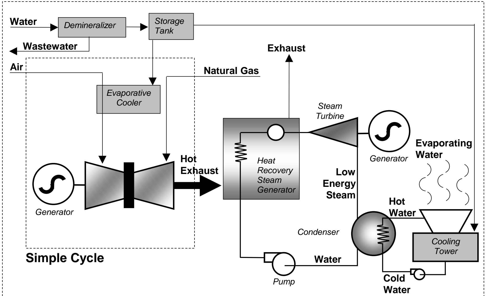
Figure 2: Simple Cycle and Combined Cycle Combustion Turbine Power Plant
